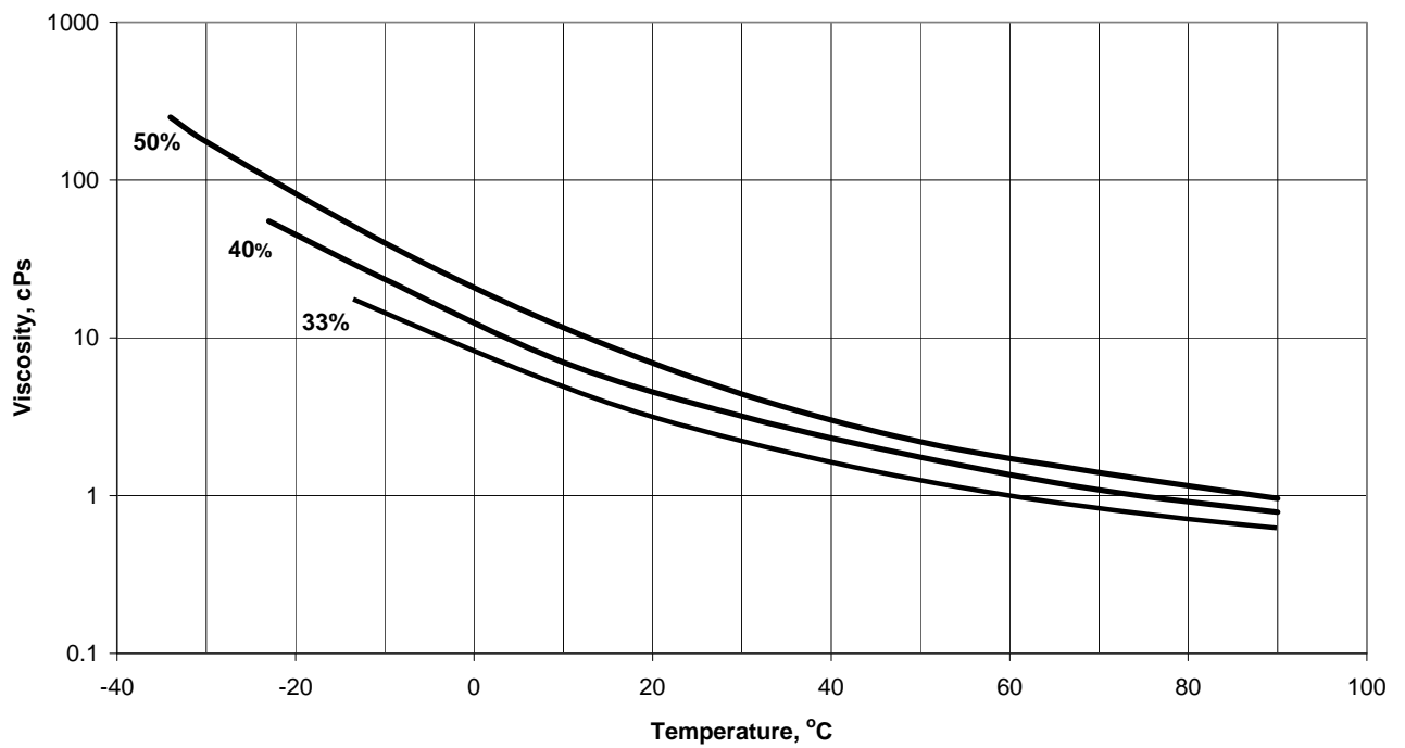
Viscosity Chart
